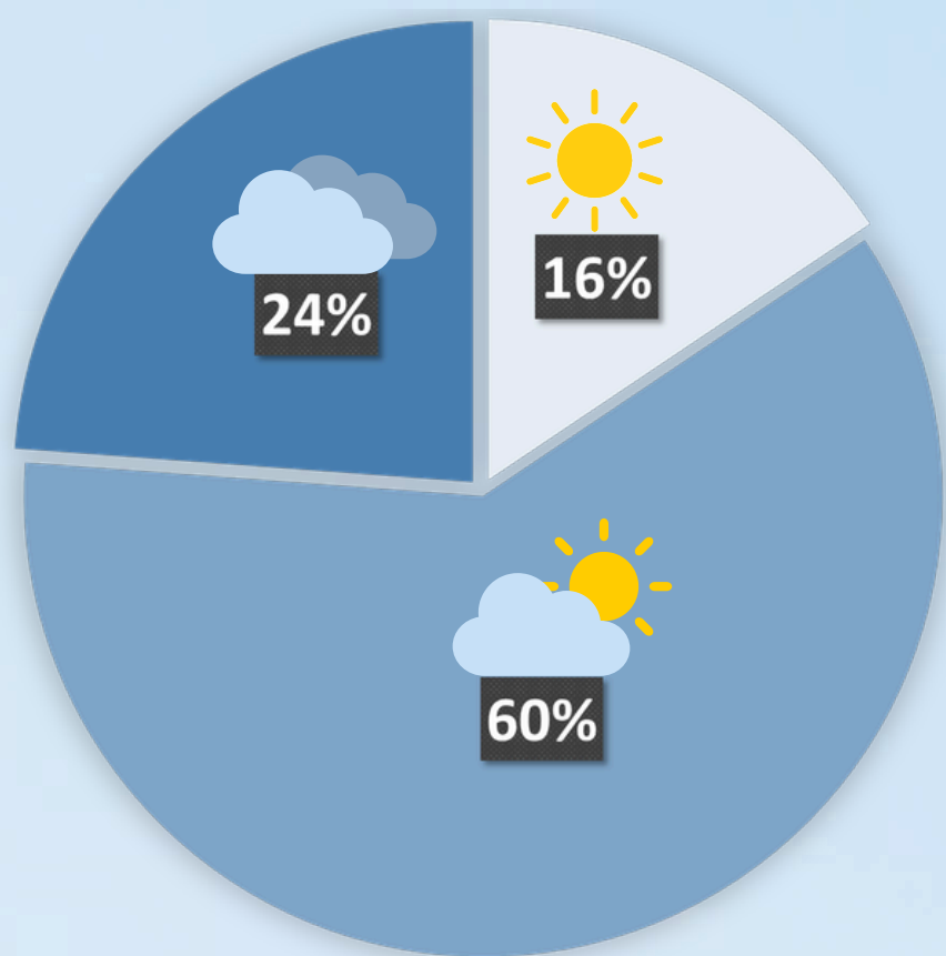
CLOUD COVER
